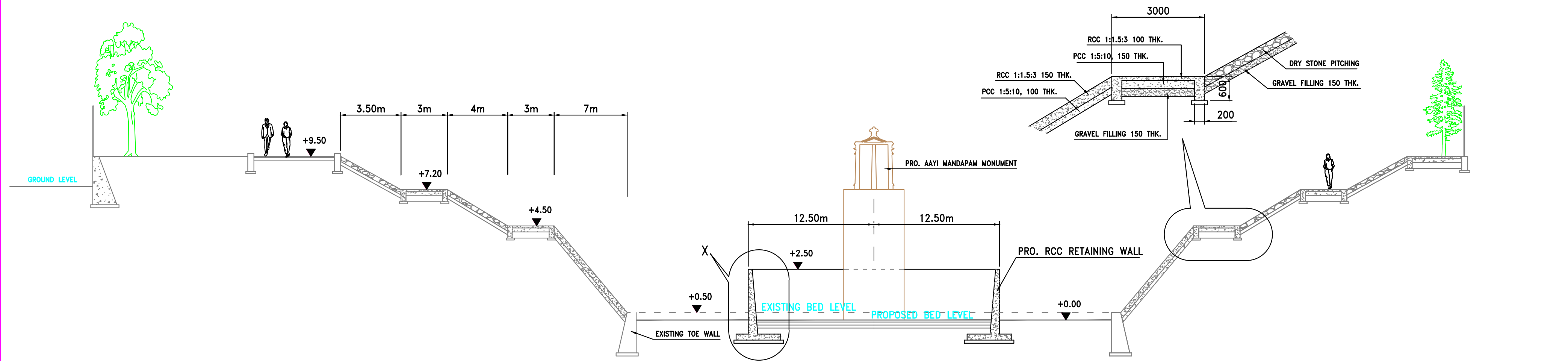
SECTION - 1-1
