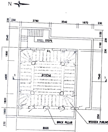
BASEMENT PLAN
