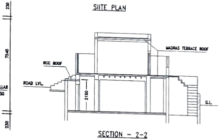
SECTION - 2-2
