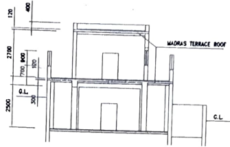
SECTION - 1-1
